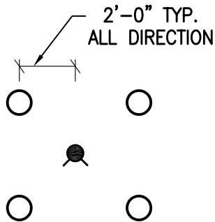
FIRE HYDRANT BOLLARD DETAIL
