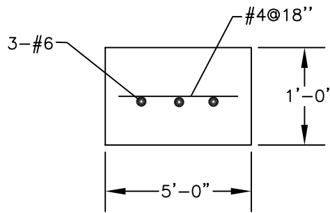
FOOTING DETAIL
